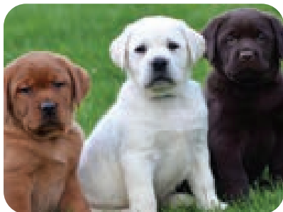
4.2-rasm. O'zgaruvchanlik
