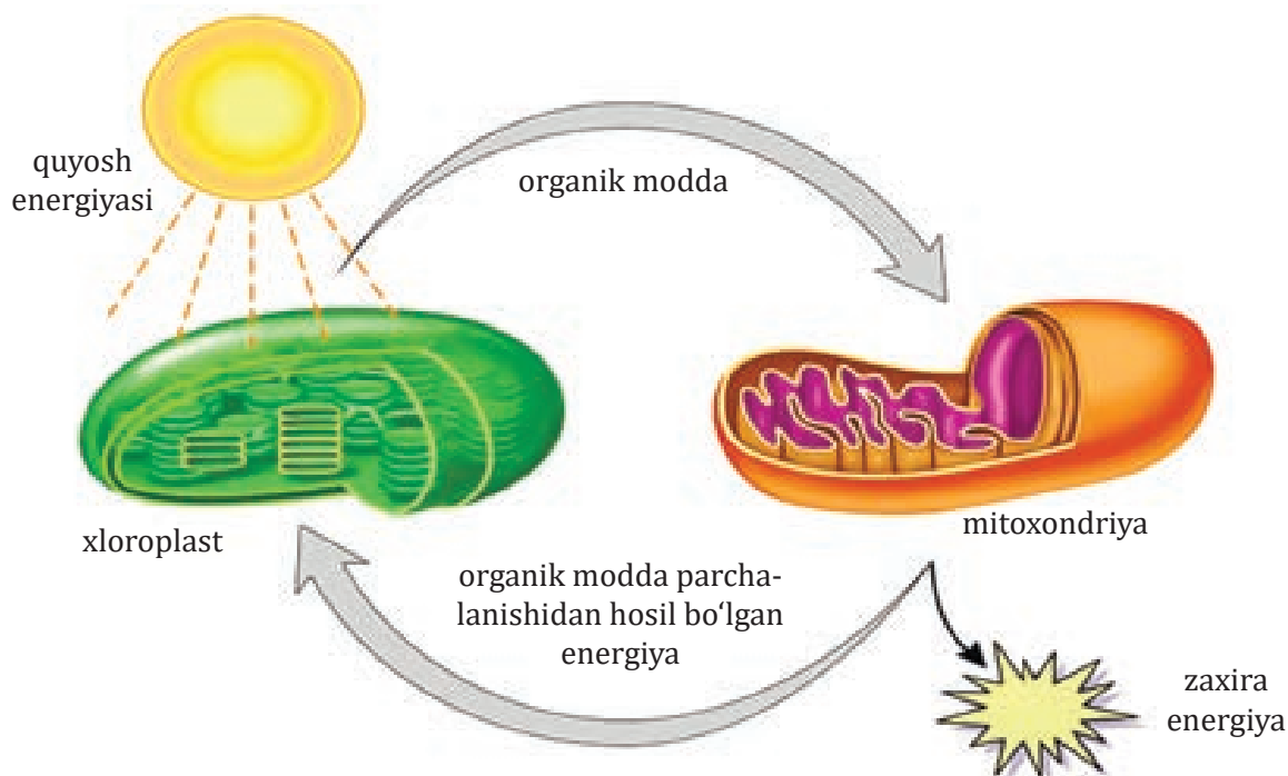
2.23-rasm. Metabolizm
