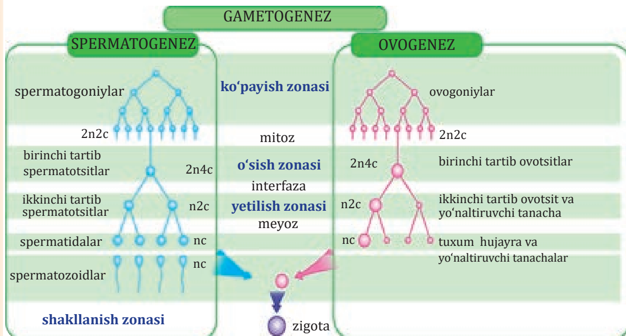
3.23-rasm. Gametogenez
