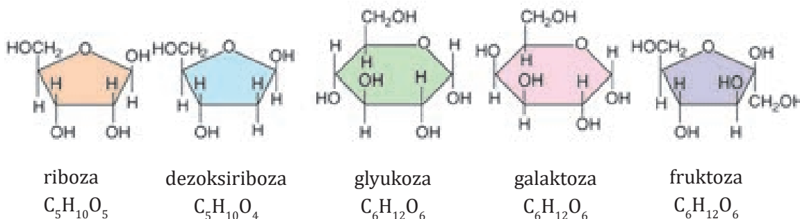
1.8-rasm. Monosaxaridlar
